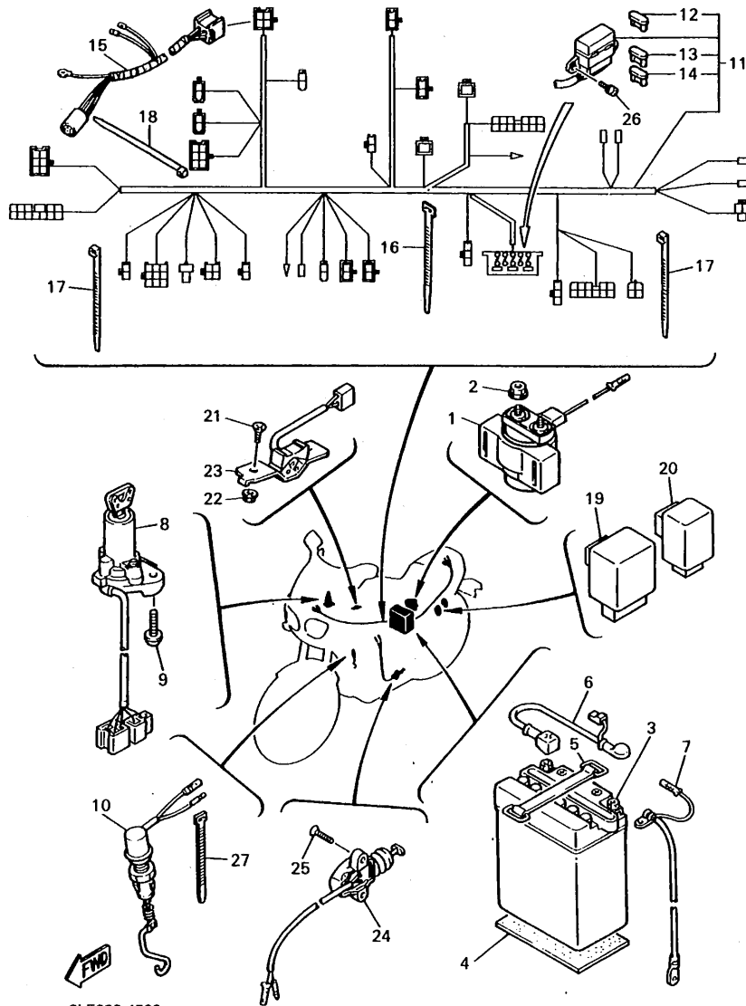
REF. NO. PART NO. DESCRIPTION Q'TY REMARKS 1 36Y-81940-00 STARTER RELAY ASSY 1 2 95701-06500 NUT, FLANGE 2 3 3XW-82100-00 BATTERY ASSY (YTX14-BS) 1 4 5Y1-82122-00 SEAT, BATTERY 1 5 2T4-82131-00 BAND, BATTERY 1 6 3GM-82115-50 WIRE, PLUS LEAD 1 7 3XW-82116-00 WIRE, MINUS LEAD 1 8 4JH-82501-00 MAIN SWITCH STEERING LOCK 1 UR 4NA-82501-00 MAIN SWITCH STEERING LOCK 1 UR FOR OCEANIA 9 90109-080G5 BOLT 2 10 3GM-82530-11 STOP SWITCH ASSY 1 11 3GM-82590-30 WIRE HARNESS ASSY 1 UR 3LK-82590-20 WIRE HARNESS ASSY 1 UR FOR OCEANIA 12 1AE-82151-00 .FUSE (30A-BL) 2 13 42X-82151-00 .FUSE (10A-BL) 4 14 2GH-82151-00 .FUSE (20A-BL) 2 15 3GM-82509-00 WIRE, SUB LEAD 1 16 90464-13080 CLAMP 2 17 90464-13073 CLAMP 7 18 25G-83936-01 BAND, SWITCH CORD 2 19 3EN-81950-00 RELAY ASSY 1 20 4BH-8195A-00 RELAY ASSY 1 21 98780-05016 SCREW, FLAT HEAD 2 22 95701-05500 NUT, FLANGE 2 23 3TJ-83964-00 SWITCH 1 24 2KT-82566-01 SWITCH, SIDE STAND 1 25 90152-05021 SCREW, COUNTERSUNK 2 26 90159-06033 SCREW, WITH WASHER 2
